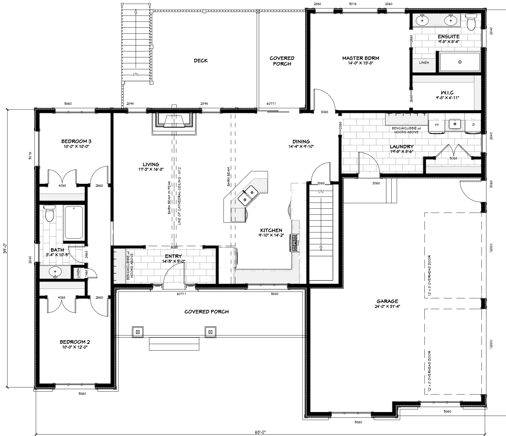
GROUND FLOOR PLAN = 1770 SQ.FT.
