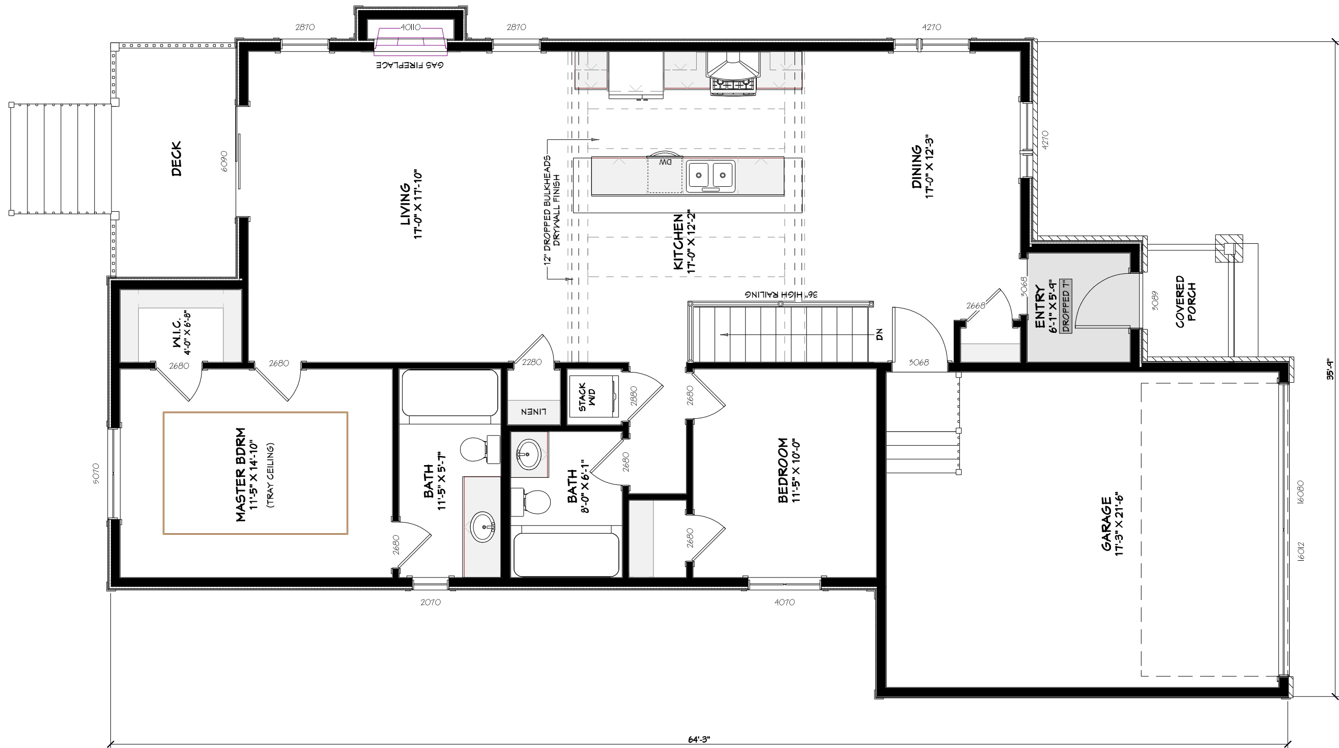
GROUND FLOOR PLAN = 1350 SQ.FT.
